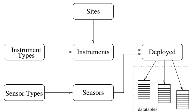
Figure 5: The REINAS Lite Schema
