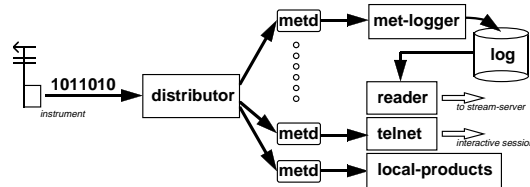
Figure 2: Instrument Node Data Flow
