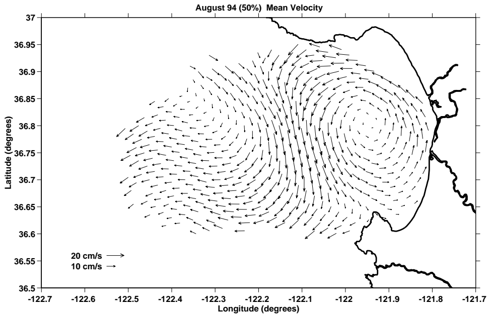
Figure 4: Sample Derived CODAR Vector Data
